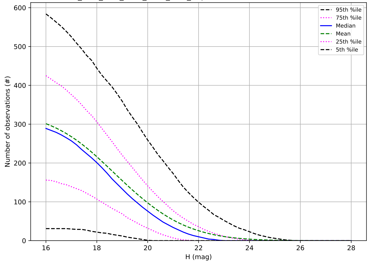
ddf_acor_sf15_lsf20_lsr10_v3.4_10yrs: Number of observations NEO
