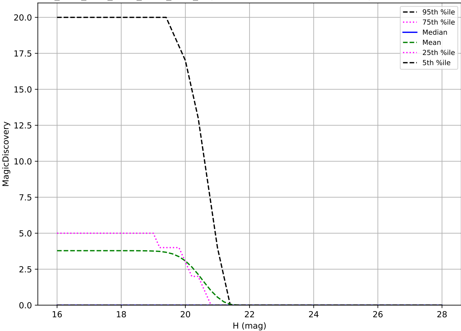
ddf_acor_sf15_lsf20_lsr10_v3.4_10yrs: Vatra 6 detections in 60 nights detection loss
