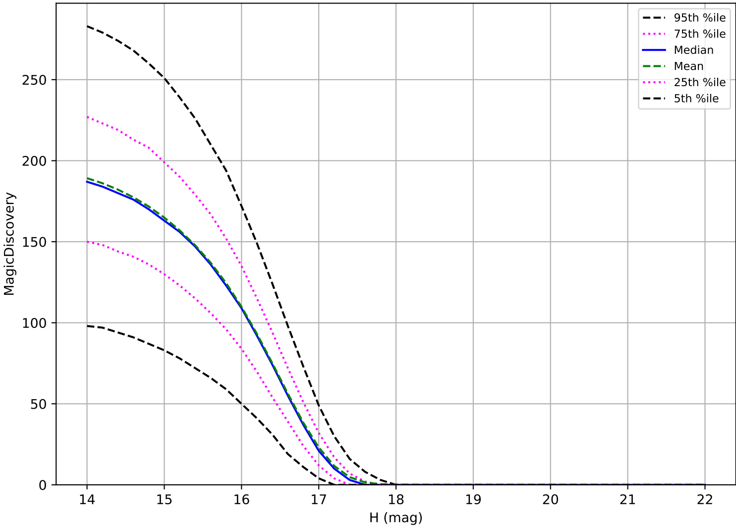
ddf_acor_sf15_lsf20_lsr10_v3.4_10yrs: Trojan 6 detections in 60 nights detection loss
