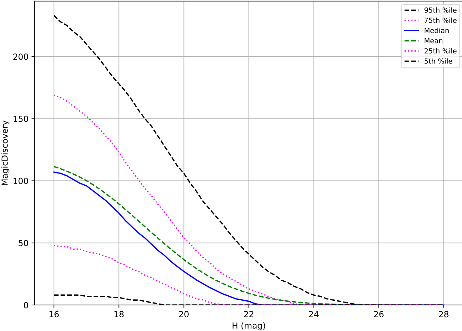
ddf_acor_sf15_lsf20_lsr10_v3.4_10yrs: PHA 6 detections in 60 nights detection loss
