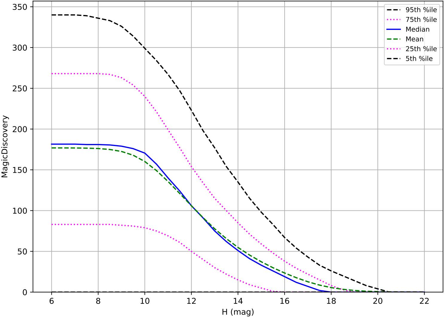
ddf_acor_sf15_lsf20_lsr10_v3.4_10yrs: OCC_r5 6 detections in 60 nights detection loss
