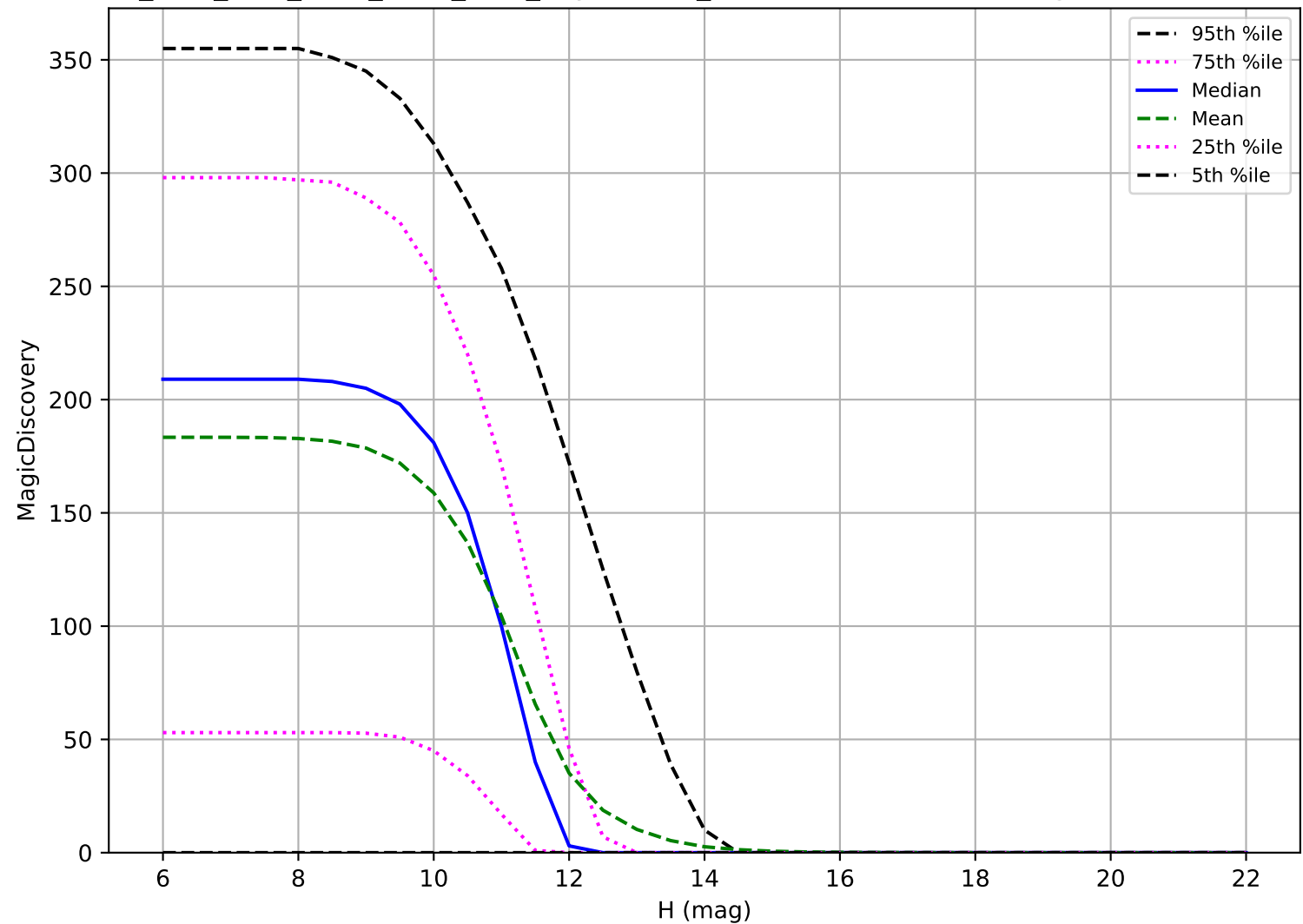
ddf_acor_sf15_lsf20_lsr10_v3.4_10yrs: OCC_r20 6 detections in 60 nights detection loss
