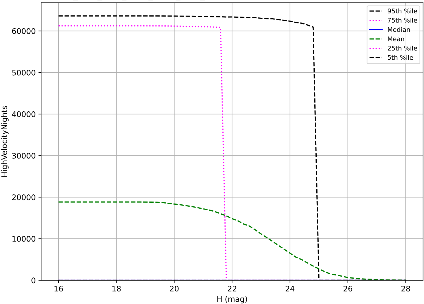
ddf_acor_sf15_lsf20_lsr10_v3.4_10yrs: NEO High velocity pair detection loss
