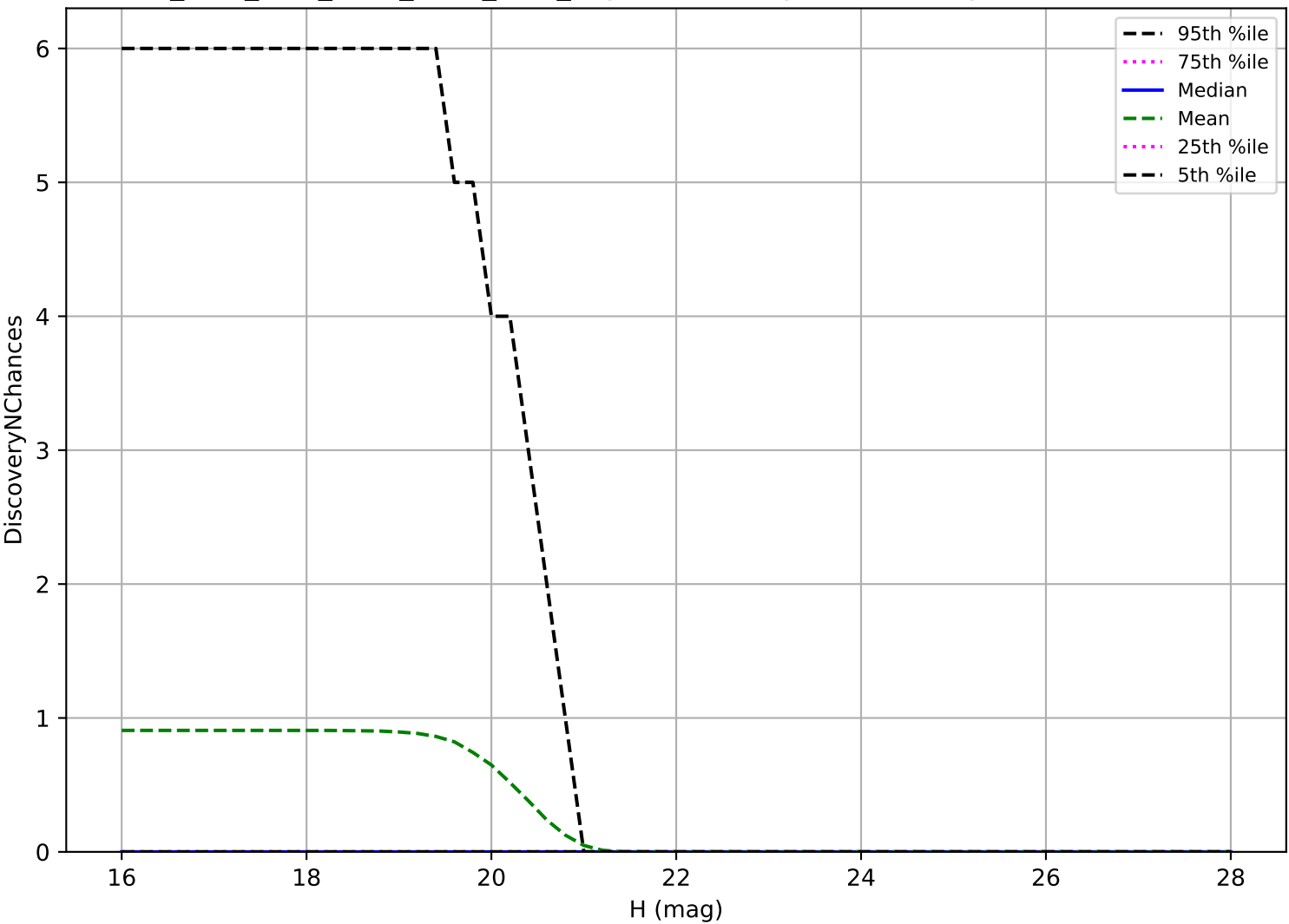
ddf_acor_sf15_lsf20_lsr10_v3.4_10yrs: Vatira 3 pairs in 15 nights detection loss
