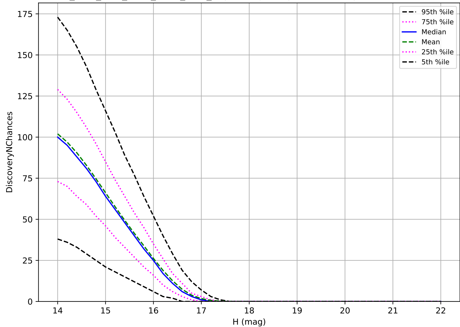
ddf_acor_sf15_lsf20_lsr10_v3.4_10yrs: Trojan 3 pairs in 15 nights detection loss
