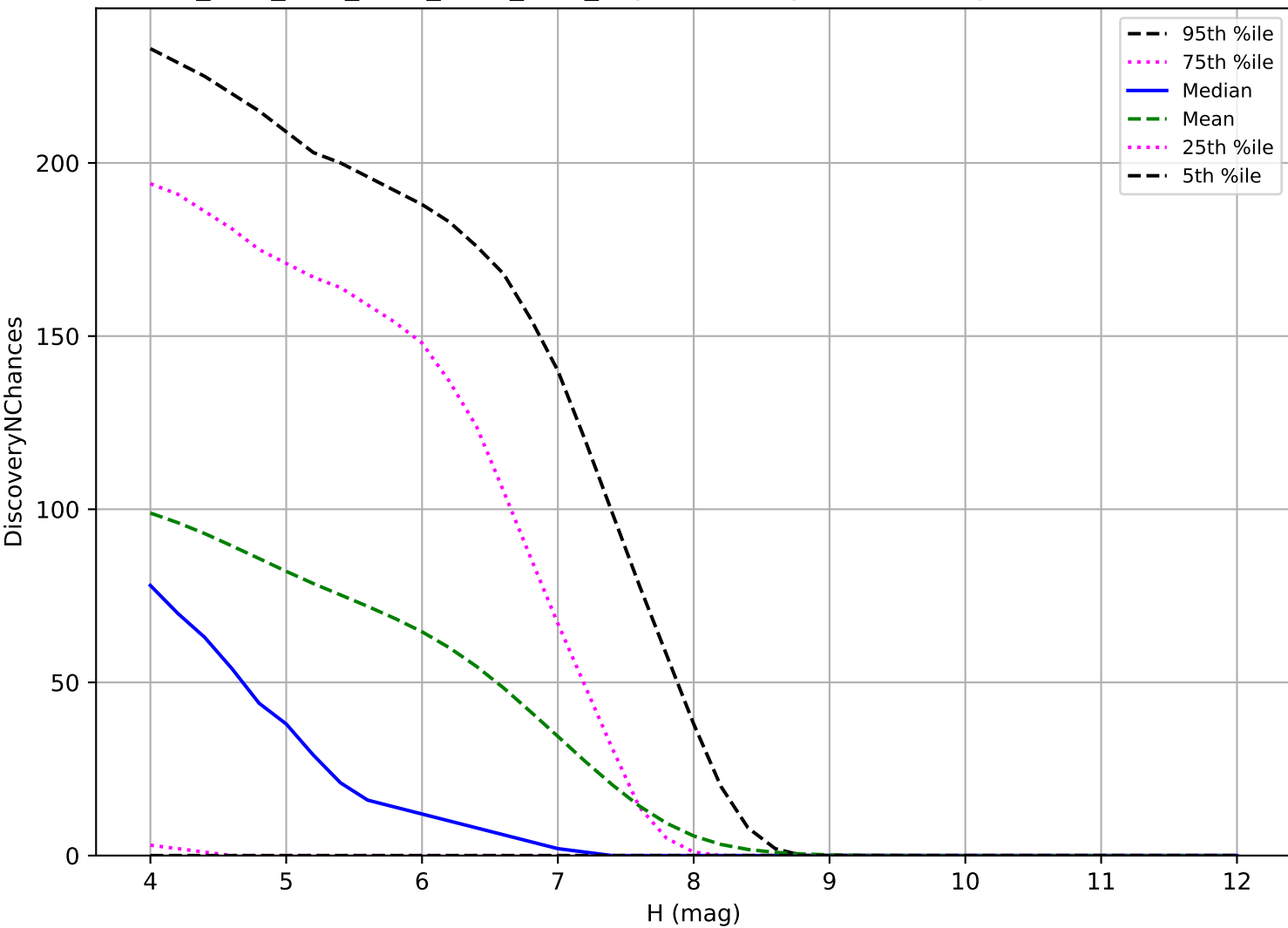
ddf_acor_sf15_lsf20_lsr10_v3.4_10yrs: TNO 3 pairs in 15 nights detection loss
