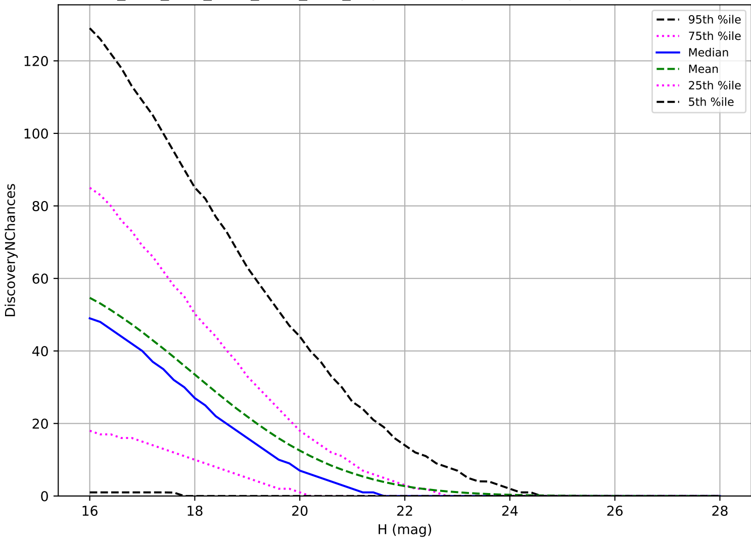
ddf_acor_sf15_lsf20_lsr10_v3.4_10yrs: PHA 3 pairs in 15 nights detection loss
