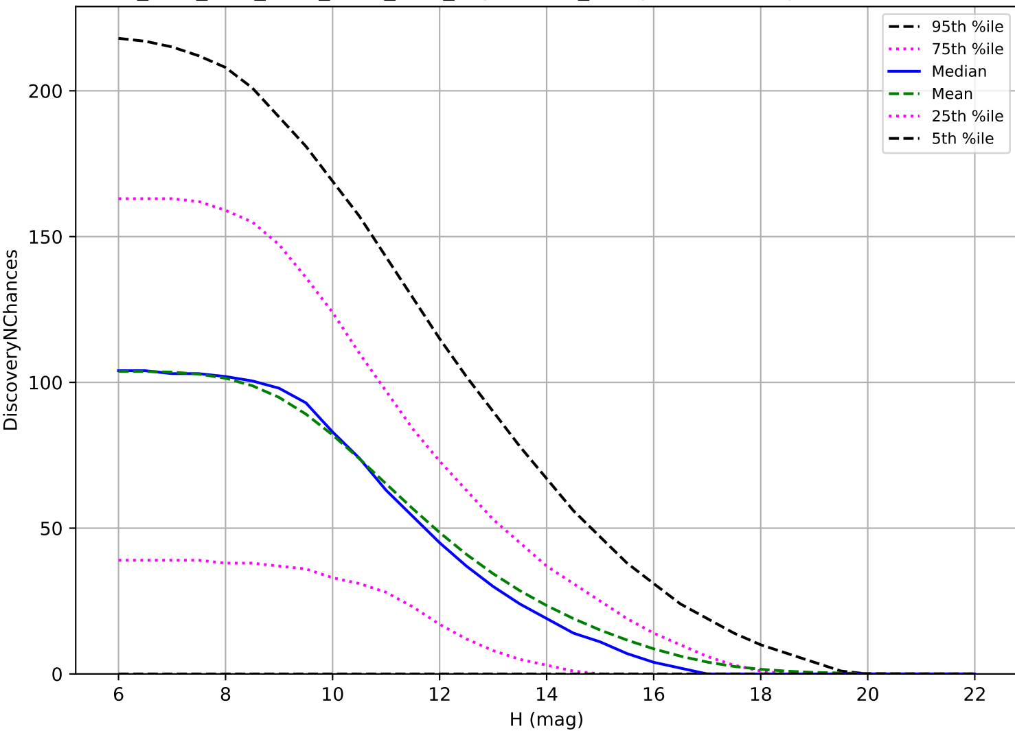
ddf_acor_sf15_lsf20_lsr10_v3.4_10yrs: OCC_r5 3 pairs in 15 nights detection loss
