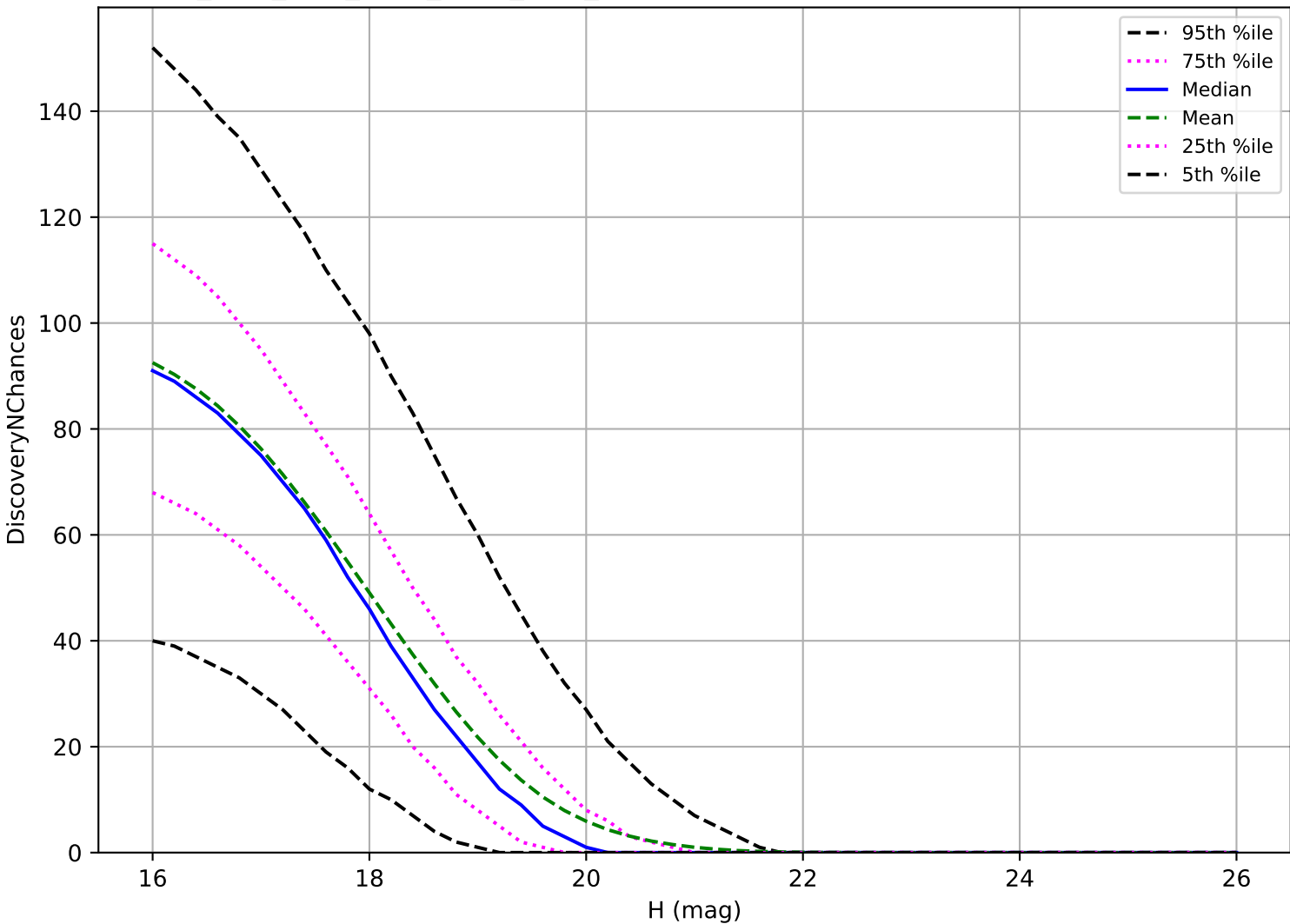
ddf_acor_sf15_lsf20_lsr10_v3.4_10yrs: MBA 3 pairs in 15 nights detection loss
