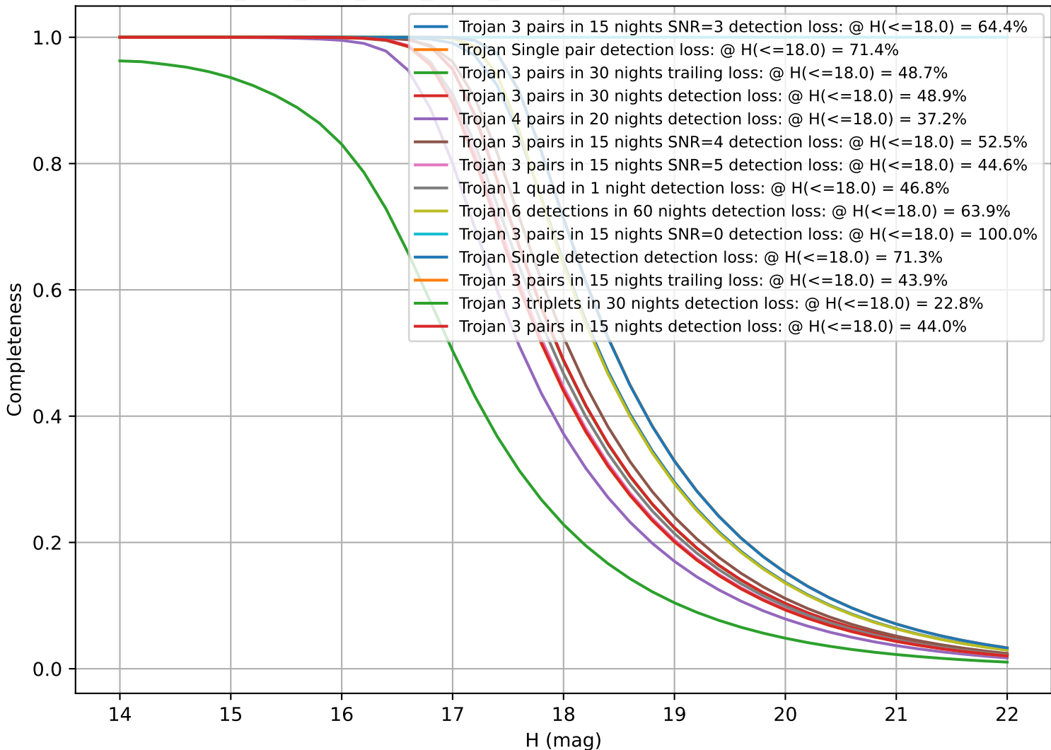
ddf_acor_sf15_lsf20_lsr10_v3.4_10yrs: CumulativeCompleteness
