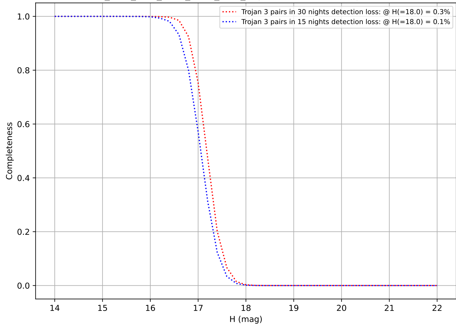
ddf_acor_sf15_lsf20_lsr10_v3.4_10yrs: DifferentialCompleteness
