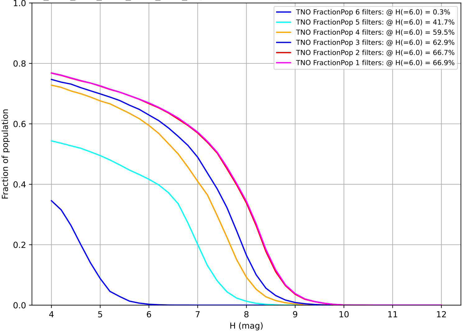
ddf_acor_sf15_lsf20_lsr10_v3.4_10yrs: Fraction of population with colors in X filters TNO
