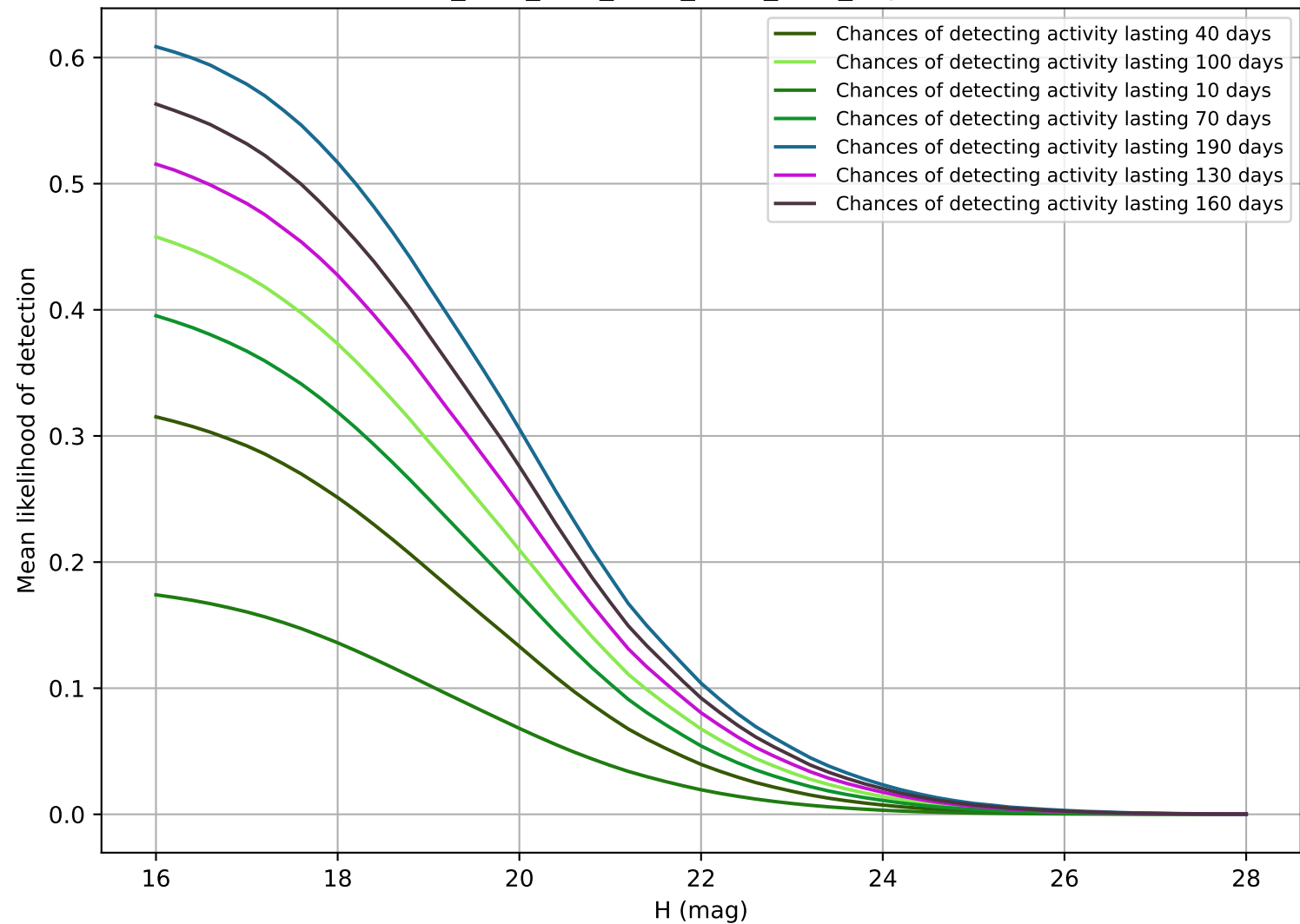
ddf_acor_sf15_lsf20_lsr10_v3.4_10yrs PHA
