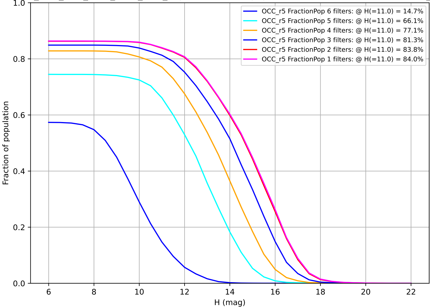
ddf_acor_sf15_lsf20_lsr10_v3.4_10yrs: Fraction of population with colors in X filters OCC_r5
