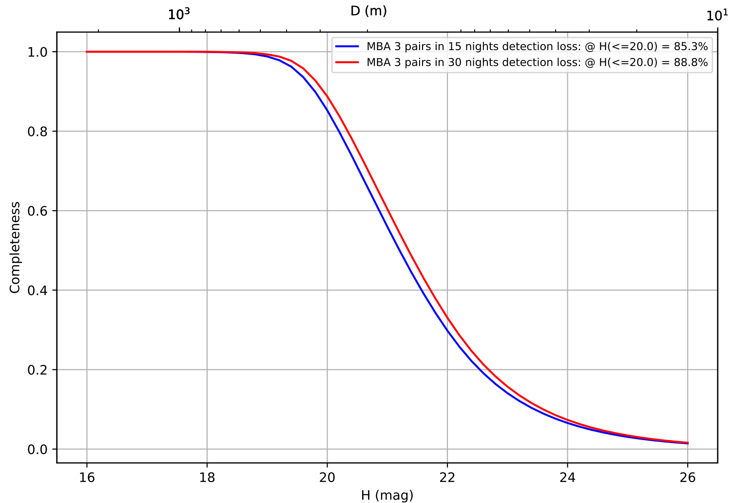
ddf_acor_sf15_lsf20_lsr10_v3.4_10yrs: CumulativeCompleteness
