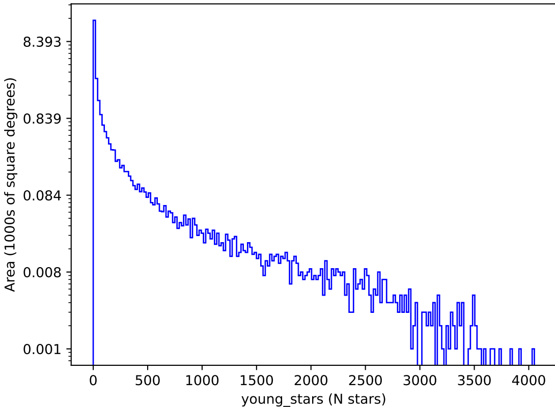
ddf_acor_sf15_lsf20_lsr10_v3.4_10yrs : young_stars
