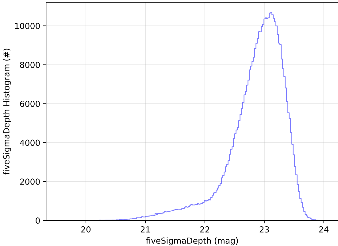
ddf_acor_sf15_lsf20_lsr10_v3.4_10yrs z: fiveSigmaDepth Histogram
