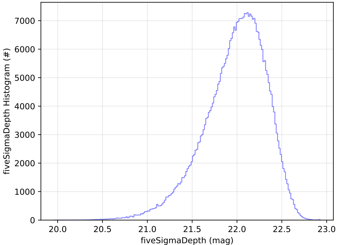
ddf_acor_sf15_lsf20_lsr10_v3.4_10yrs y: fiveSigmaDepth Histogram
