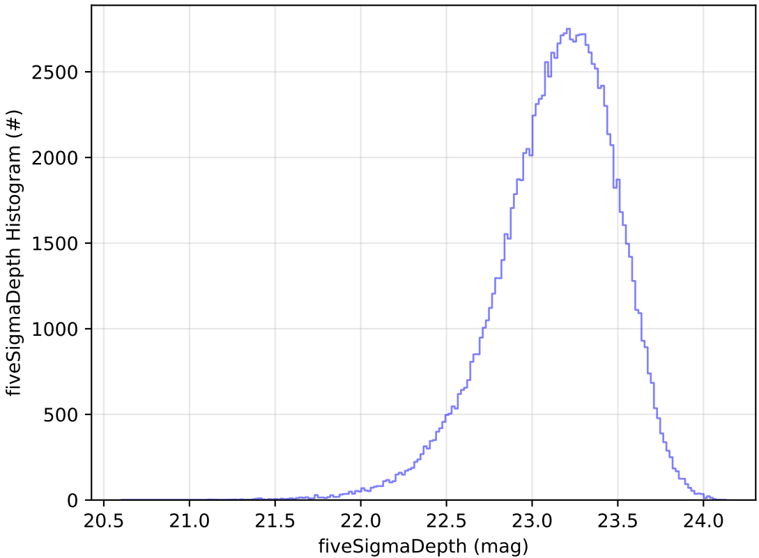
ddf_acor_sf15_lsf20_lsr10_v3.4_10yrs u: fiveSigmaDepth Histogram
