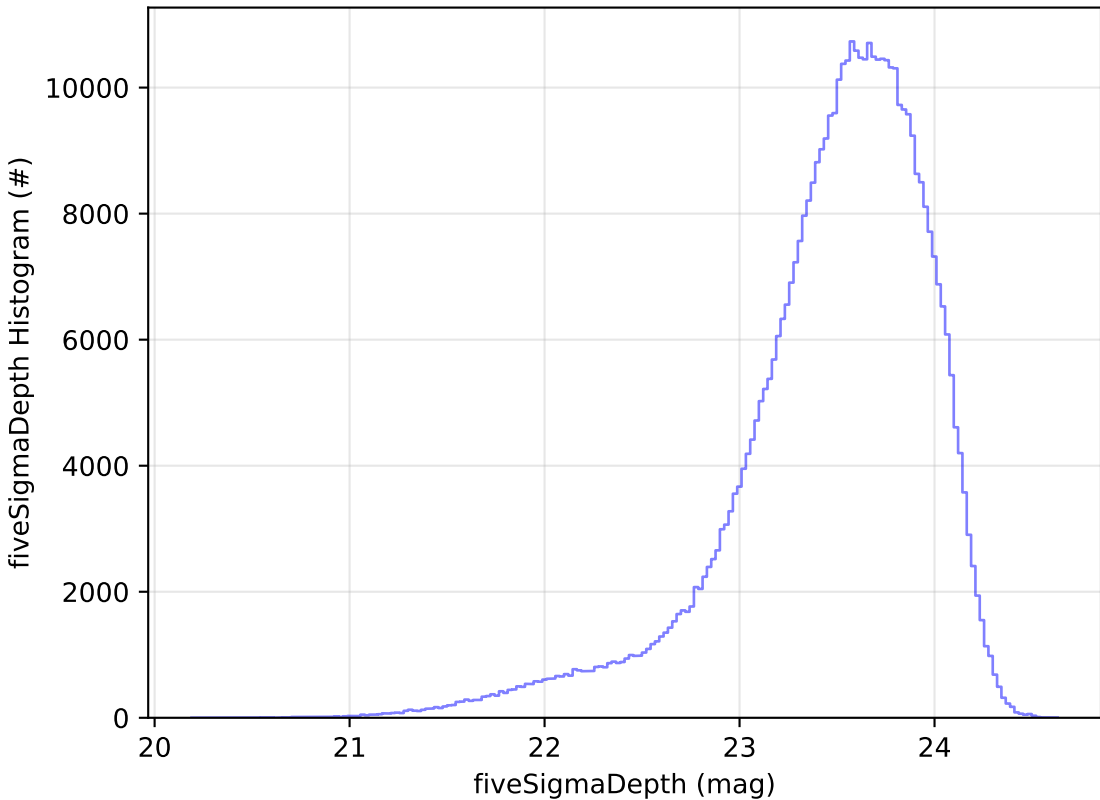
ddf_acor_sf15_lsf20_lsr10_v3.4_10yrs i: fiveSigmaDepth Histogram
