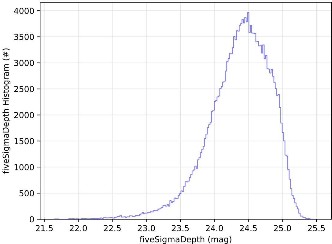
ddf_acor_sf15_lsf20_lsr10_v3.4_10yrs g: fiveSigmaDepth Histogram
