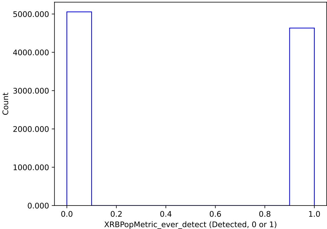
ddf_acor_sf15_lsf20_lsr10_v3.4_10yrs : XRBPoMetric_ever_detect
