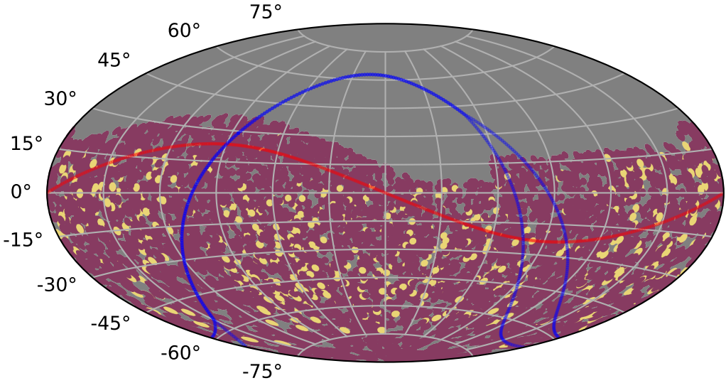
ddf_acor_sf15_lsf20_lsr10_v3.4_10yrs : TDEsPopMetric_some_color
