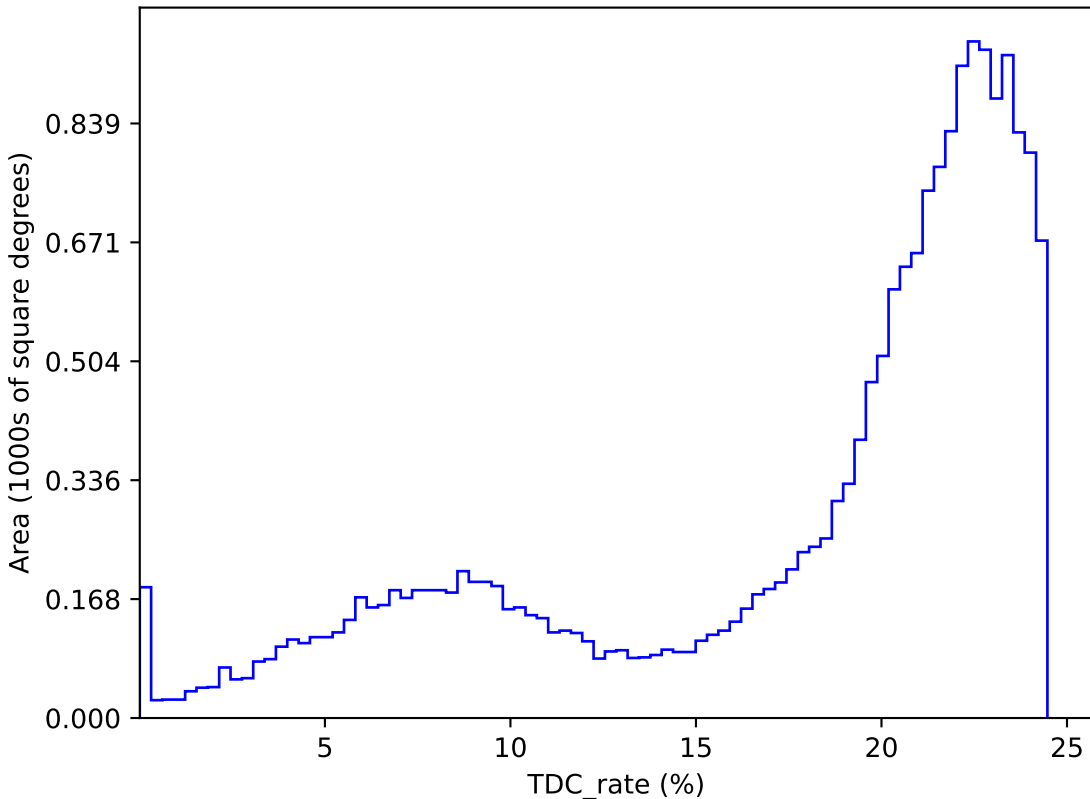
ddf_acor_sf15_lsf20_lsr10_v3.4_10yrs : TDC_rate
