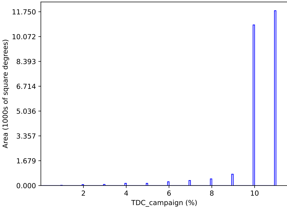
ddf_acor_sf15_lsf20_lsr10_v3.4_10yrs : TDC_campaign
