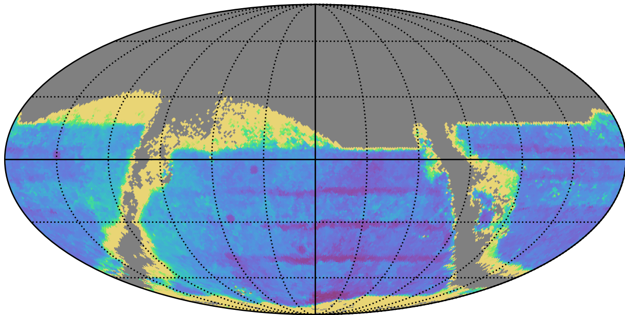
ddf_acor_sf15_lsf20_lsr10_v3.4_10yrs : TDC_accuracy
