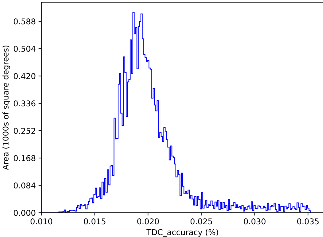
ddf_acor_sf15_lsf20_lsr10_v3.4_10yrs : TDC_accuracy
