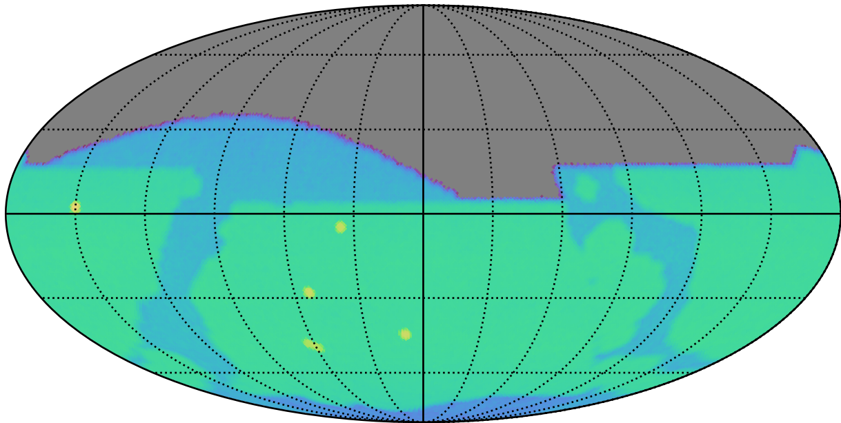
ddf_acor_sf15_lsf20_lsr10_v3.4_10yrs i: SurfaceBrightLimit
