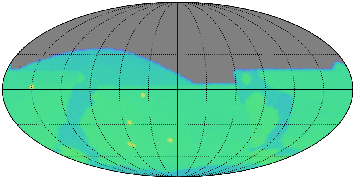
ddf_acor_sf15_lsf20_lsr10_v3.4_10yrs g: SurfaceBrightLimit
