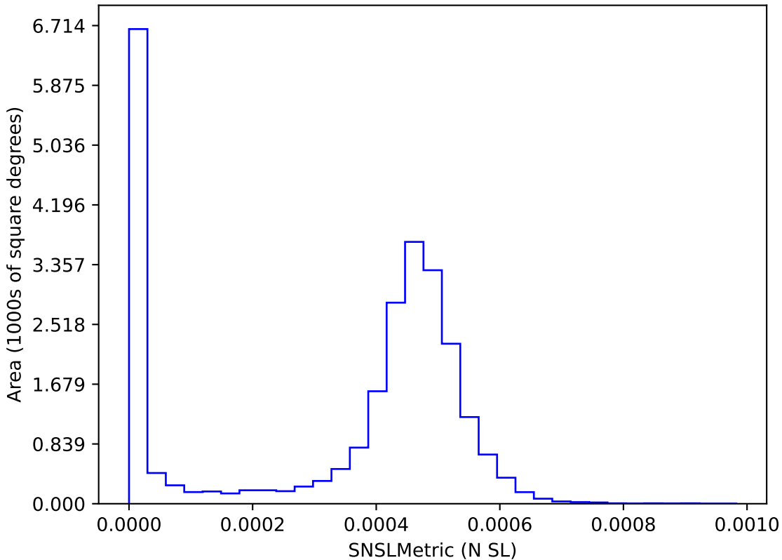
ddf_acor_sf15_lsf20_lsr10_v3.4_10yrs : SNSLMetric
