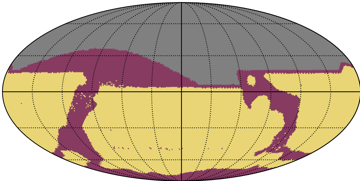
ddf_acor_sf15_lsf20_lsr10_v3.4_10yrs : RapidRevisits
