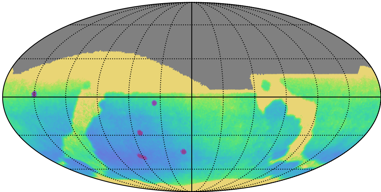
ddf_acor_sf15_lsf20_lsr10_v3.4_10yrs : Parallax Uncert @ 24.0
