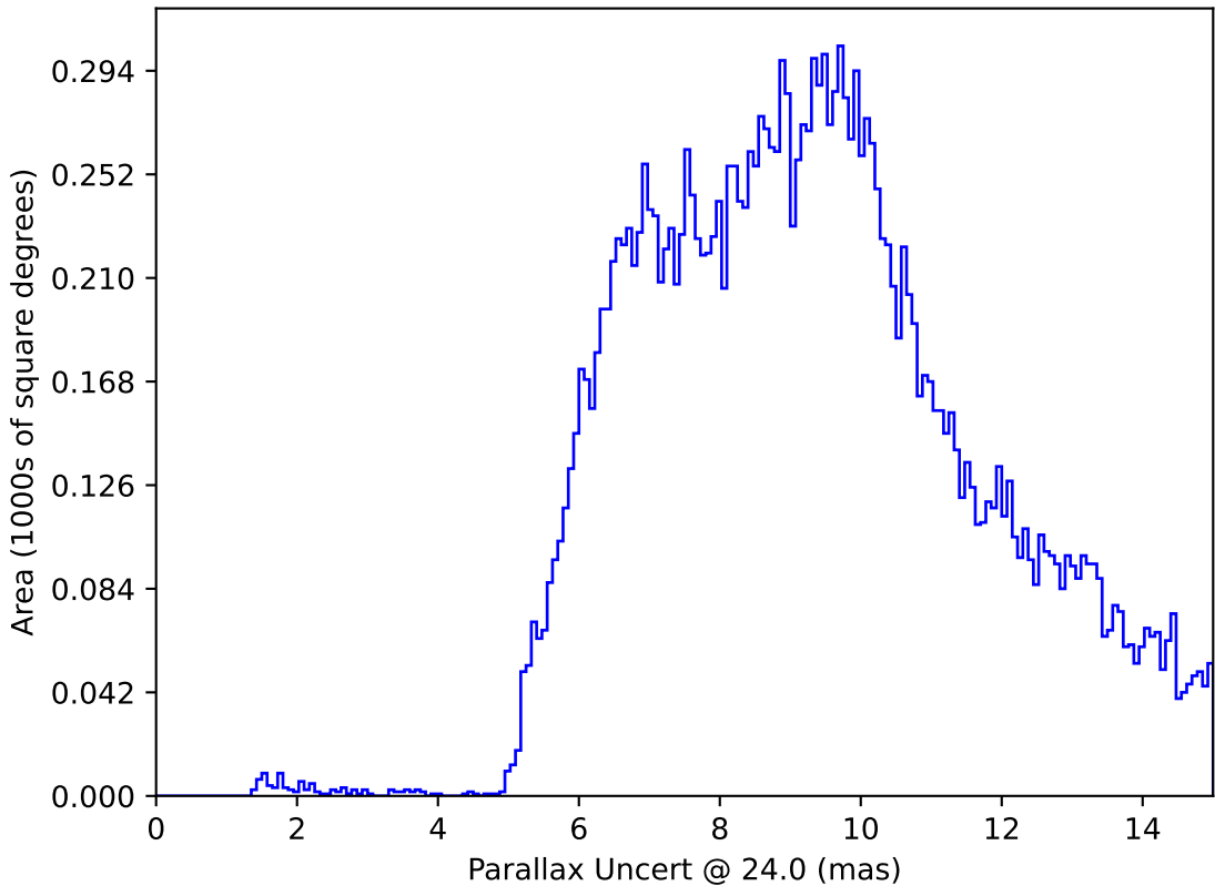
ddf_acor_sf15_lsf20_lsr10_v3.4_10yrs : Parallax Uncert @ 24.0
