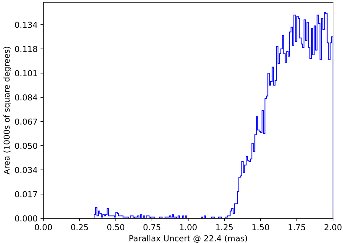
ddf_acor_sf15_lsf20_lsr10_v3.4_10yrs : Parallax Uncert @ 22.4
