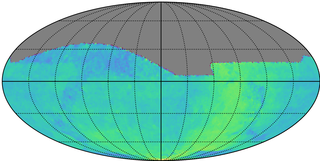
ddf_acor_sf15_lsf20_lsr10_v3.4_10yrs : Parallax Coverage @ 24.0
