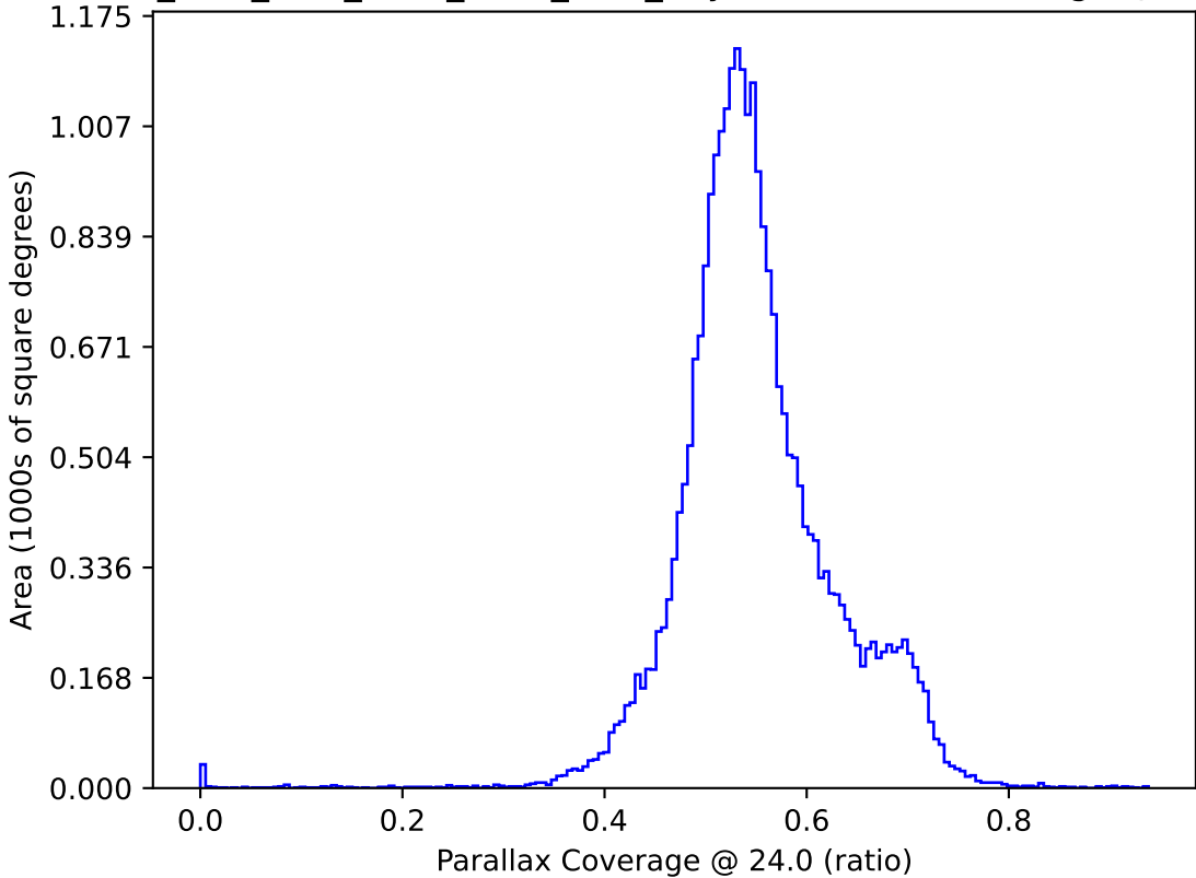
ddf_acor_sf15_lsf20_lsr10_v3.4_10yrs : Parallax Coverage @ 24.0
