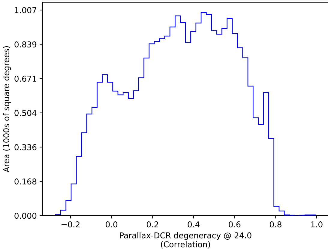
ddf_acor_sf15_lsf20_lsr10_v3.4_10yrs : Parallax-DCR degeneracy @ 24.0
