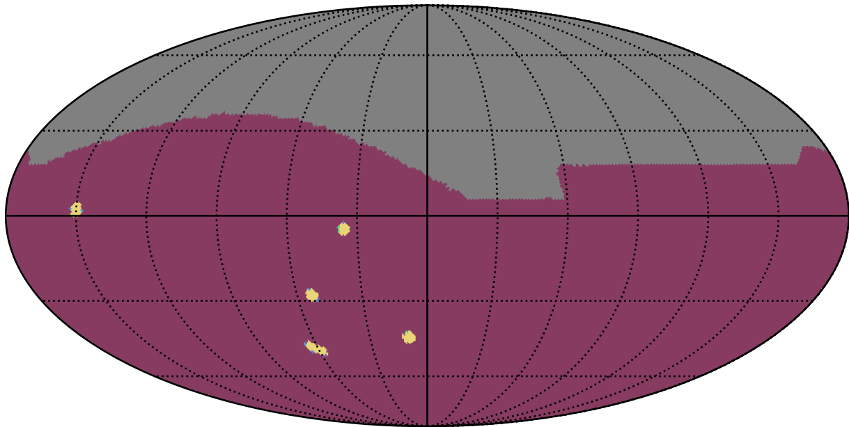
ddf_acor_sf15_lsf20_lsr10_v3.4_10yrs : NumberOfQuickRevisits
