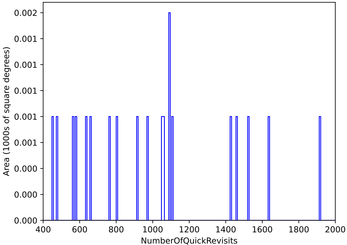
ddf_acor_sf15_lsf20_lsr10_v3.4_10yrs : NumberOfQuickRevisits
