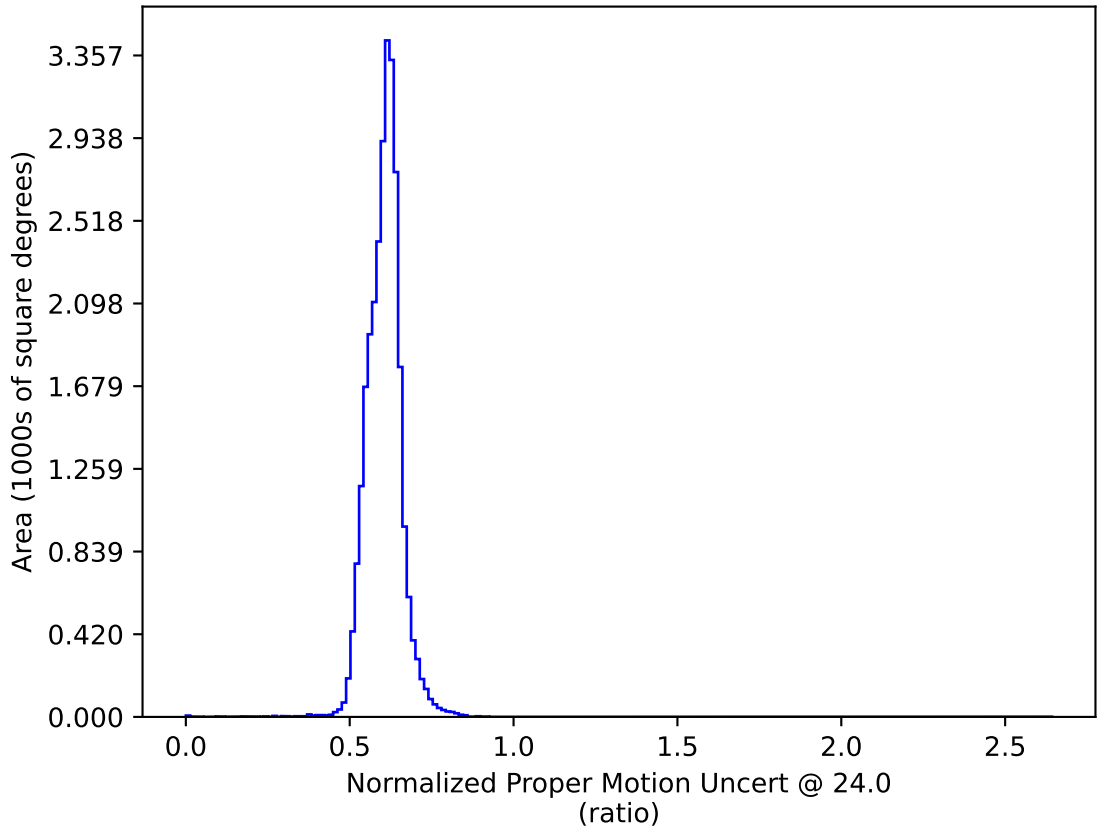
ddf_acor_sf15_lsf20_lsr10_v3.4_10yrs : Normalized Proper Motion Uncert @ 24.0
