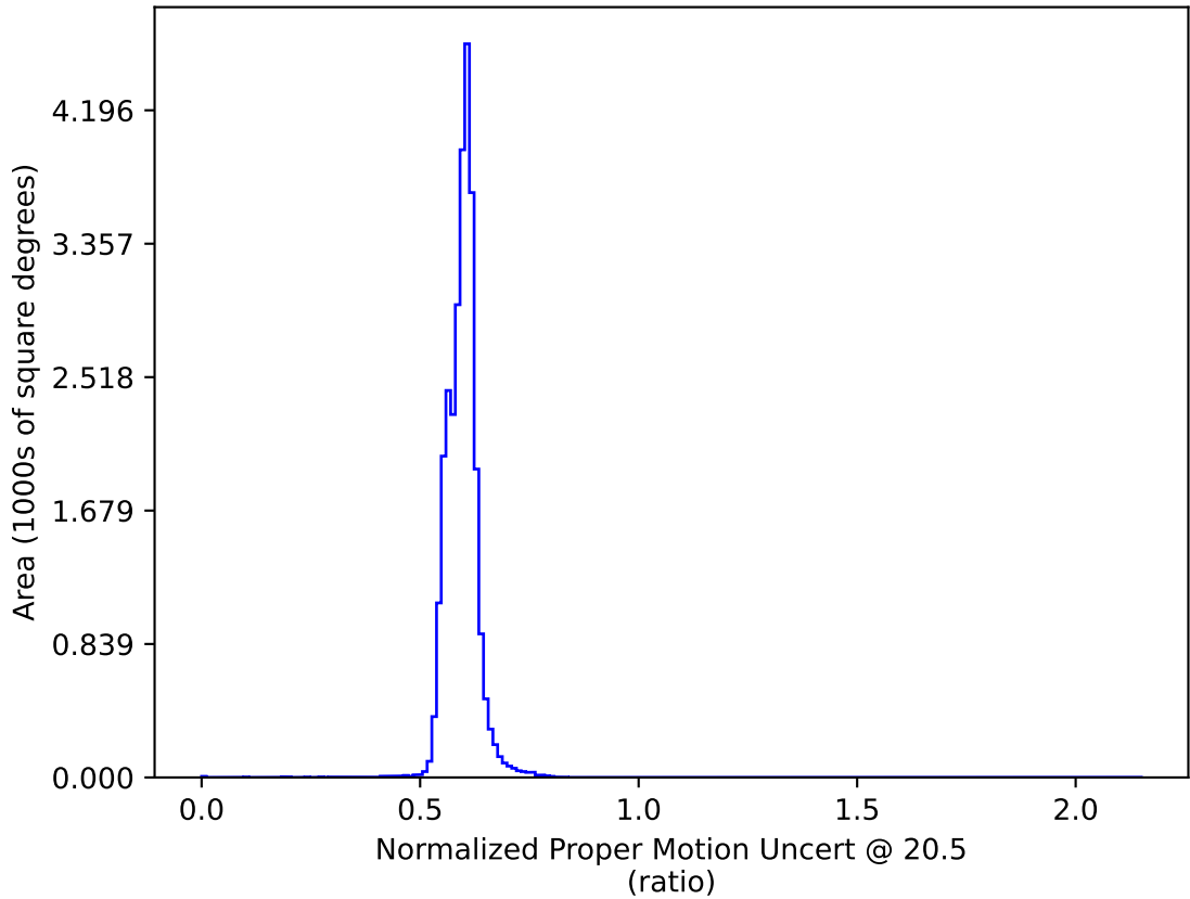
ddf_acor_sf15_lsf20_lsr10_v3.4_10yrs : Normalized Proper Motion Uncert @ 20.5
