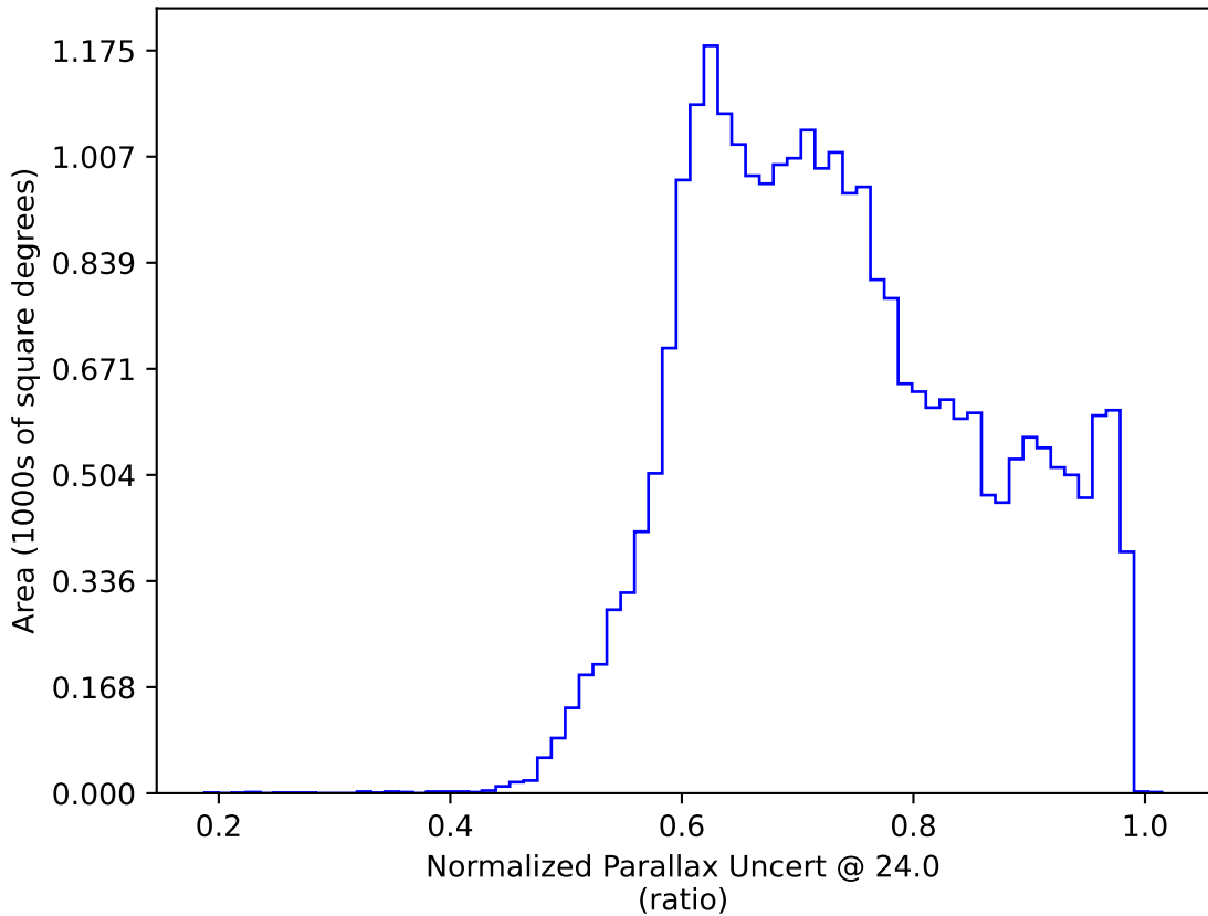
ddf_acor_sf15_lsf20_lsr10_v3.4_10yrs : Normalized Parallax Uncert @ 24.0
