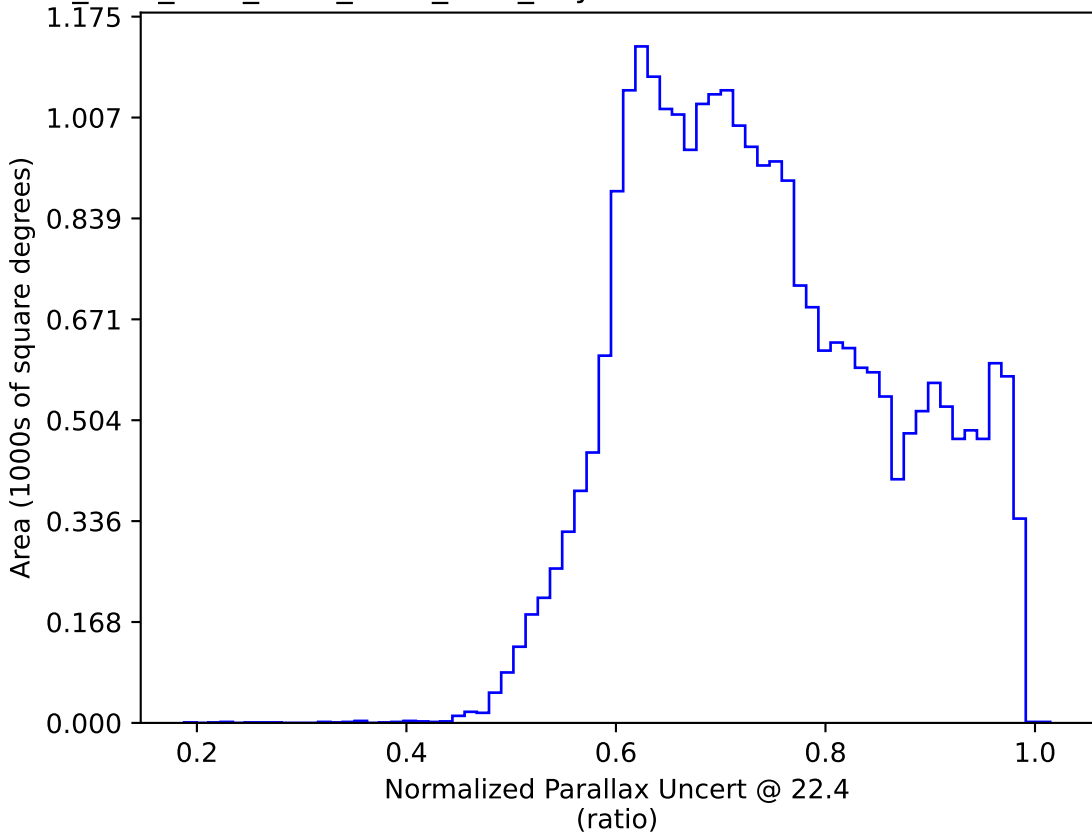
ddf_acor_sf15_lsf20_lsr10_v3.4_10yrs : Normalized Parallax Uncert @ 22.4
