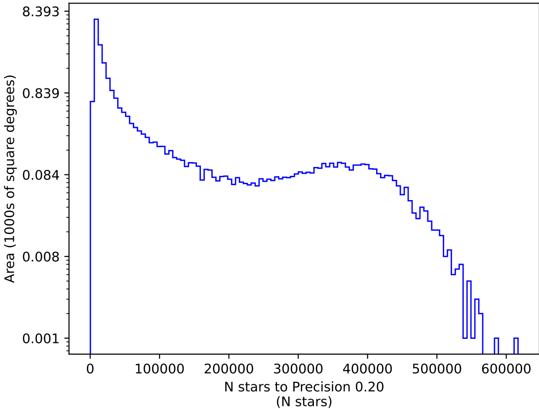
ddf_acor_sf15_lsf20_lsr10_v3.4_10yrs y: N stars to Precision 0.20
