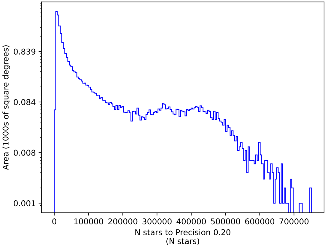
ddf_acor_sf15_lsf20_lsr10_v3.4_10yrs r: N stars to Precision 0.20
