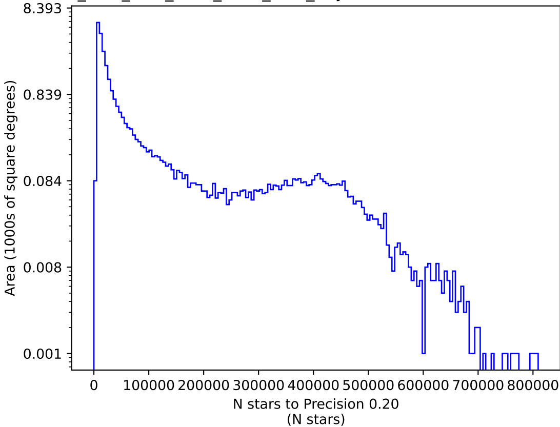
ddf_acor_sf15_lsf20_lsr10_v3.4_10yrs i: N stars to Precision 0.20
